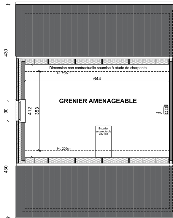
Plan grenier
