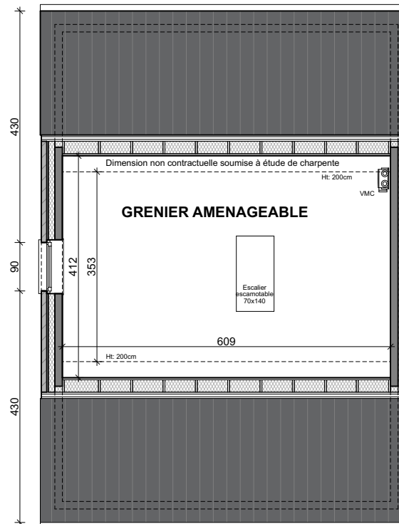
Plan grenier
