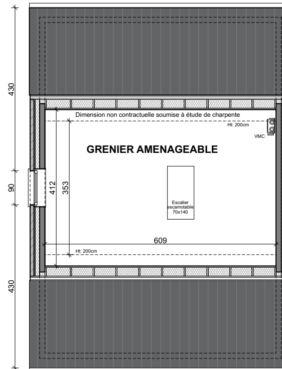
Plan grenier
